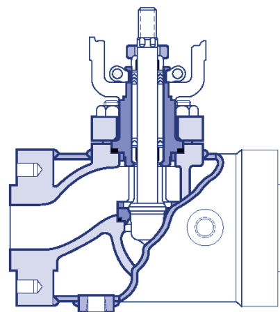
Figure 6: Steam Jacketed body configuration
