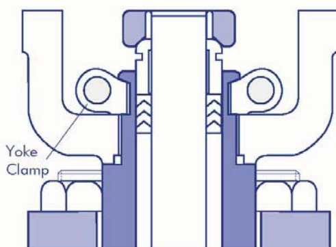
Figure 10: Yoke Clamp
