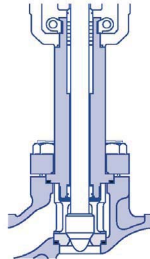
Cold Box Extended Bonnet
