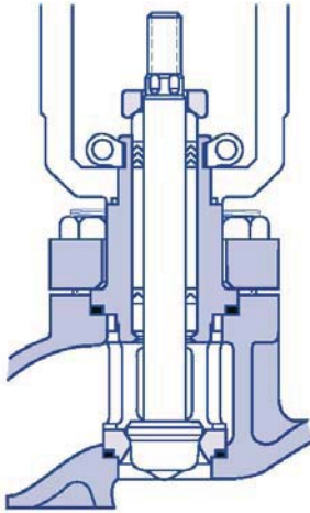
Standard Bonnet
