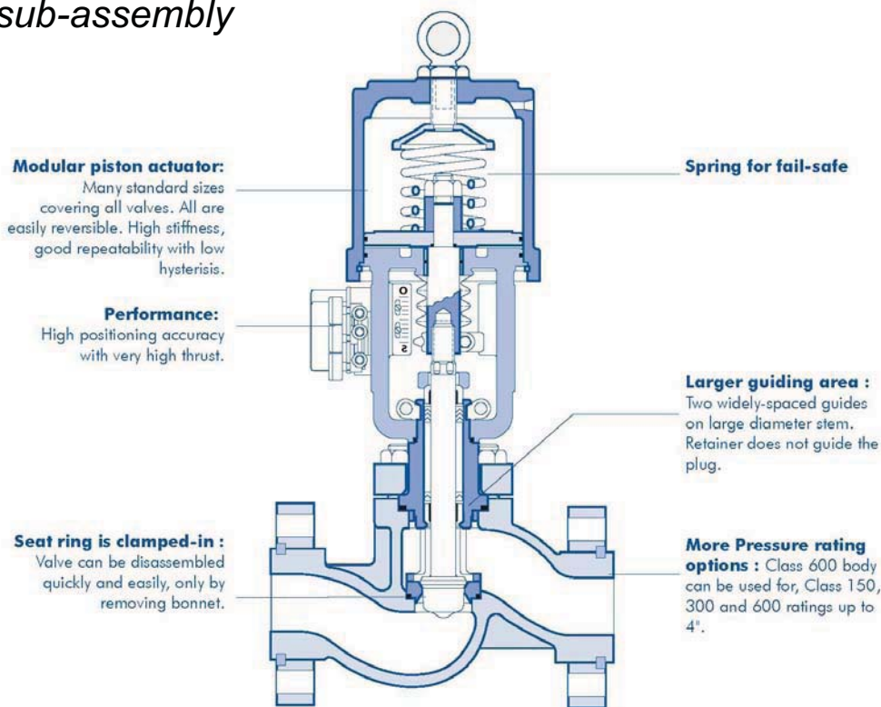
Figure 1: GFlo Body Assembly, Class 150, 300, and 600
