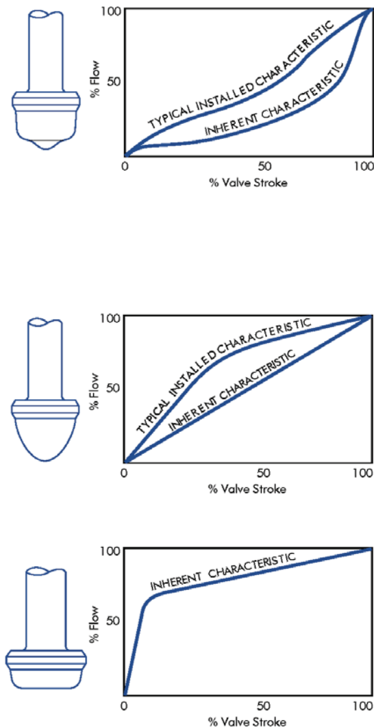
Figure 13: Flow Characteristics
