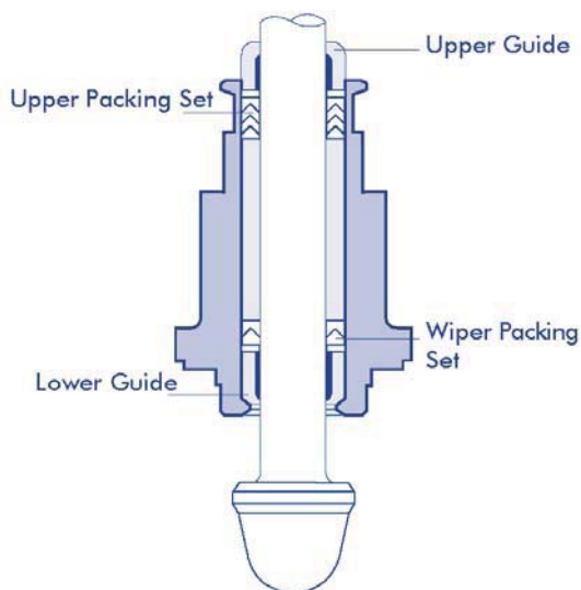
Figure 12: Typical Teflon V-ring Arrangement
