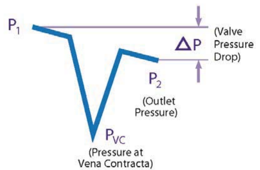
Pressure Profile Single Seat
