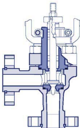
Figure 5: Angle-style body configuration
