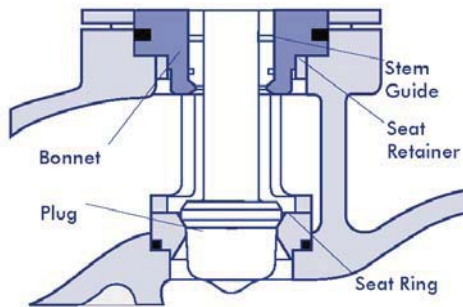
Figure 15: Standard Trim
