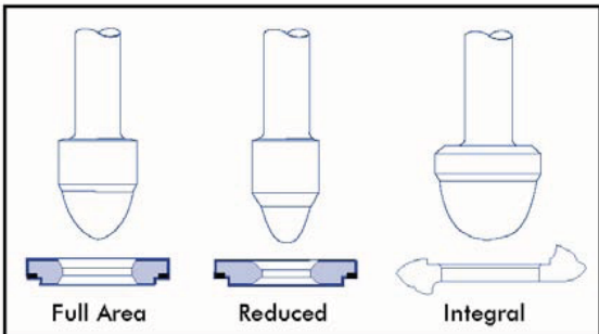
Figure 14: Typical Trim Types
