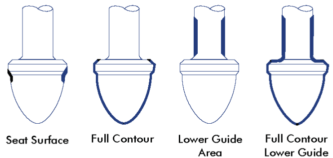
Figure 18: Hard Facing Variations-Plug
