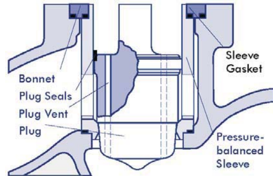
Figure 16: Pressure-balanced Trim
